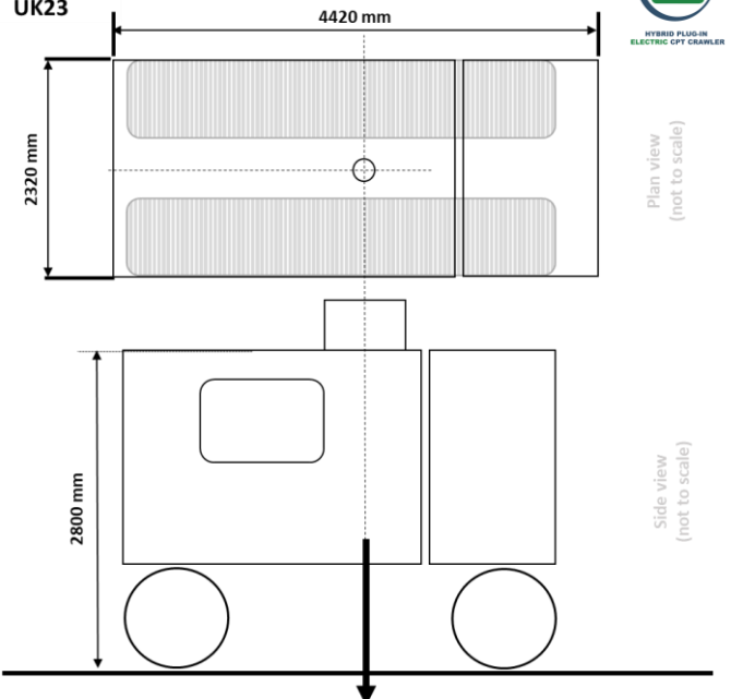
PLUG-IN HYBRID ELECTRIC CPT CRAWLER UK23
